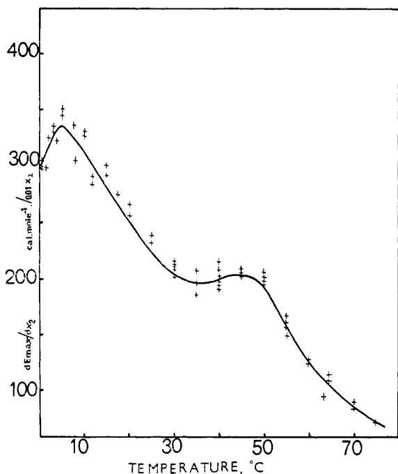
Figure 7. dE_{\max}/dx_2 as a function of temperature, from ref 368, for iodide ( 5 \times 10^{-5} M ) in aqueous t -butyl alcohol mixtures.
