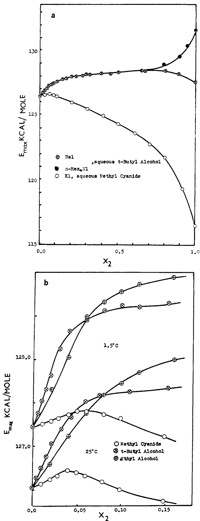
Figure 3. (a) E_{max} as a function of solvent system composition at 1.5 and 25°, for iodide ( 5 \times 10^{-6} M ) (from ref 374). (b) E_{max} as a function of solvent system composition in the highly aqueous region 0.0 < x_2 < 0.15 .
