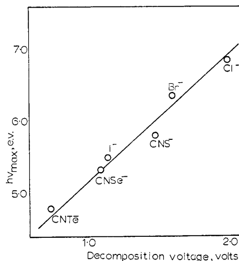
Figure 9. E_{\max} (in electron volts) as a function of the decomposition voltage of halide and pseudo-halide ions in 0.1 M salt solution (from ref 89 by kind permission of the authors).
