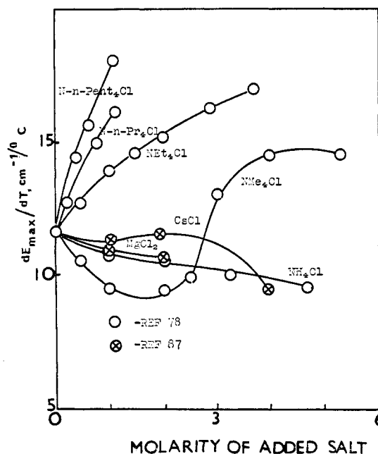
Figure 6. dE_{\text{max}}/dT as a function of added salt for iodide ( \sim 5 \times 10^{-5} M) (from ref 78 and 87).
