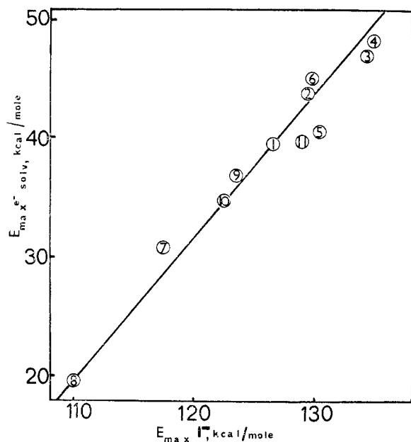
Figure 5. Plot of E_{\max} for iodide against E_{\max} for solvated electrons in a given solvent (data from ref 194 and 196). Key: (1) H 2 O; (2) MgCl 2 , 4.6 M; (3) KF, 12 M; (4) LiCl, 15 M; (5) MeOH; (6) EtOH; (7) ethylenediamine; (8) liquid ammonia ( E_{\max} for iodide extrapolated to 20°); (9) 25% NH 3 in H 2 O; (10) 12 M NH 3 in H 2 O; (11) KI crystal.
