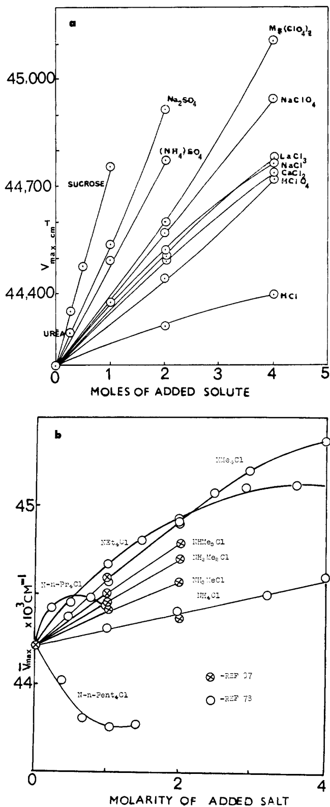
Figure 4. E_{max} as a function of added salt in water for iodide ( 5 \times 10^{-6} M ) for (a) simple inorganic salts, and (b) alkylammonium salts (from ref 78 and 87).
