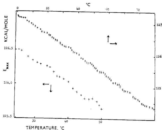
Figure 8. E_{\max} as a function of temperature for iodide ( 5 \times 10^{-5} M ) in water from 1 to 91^\circ (from ref 446).
