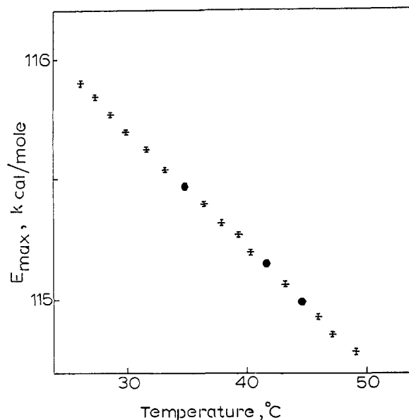
Figure 1. E_{\max} as a function of temperature for iodide ( 5 \times 10^{-5} M) in acetonitrile (from ref 445).
